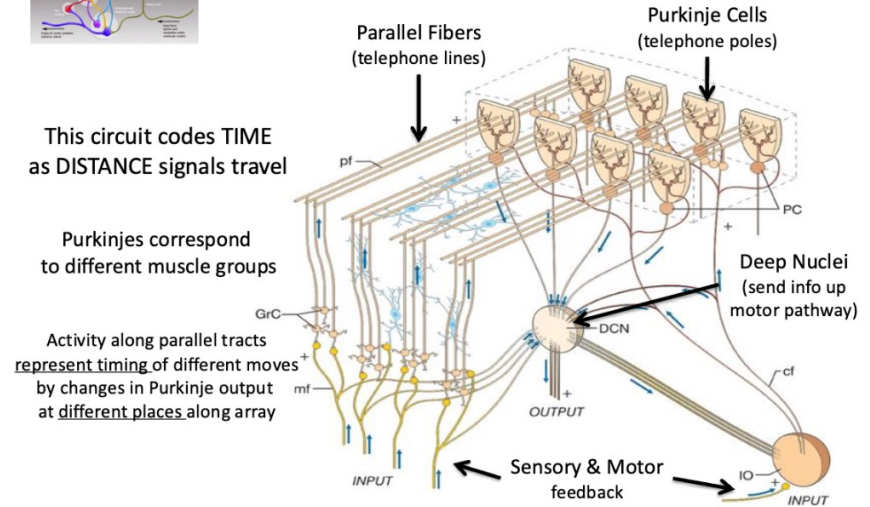
Cerebellar Circuits
